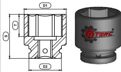
6pt. STD Socket
