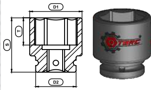
6pt. STD Socket
