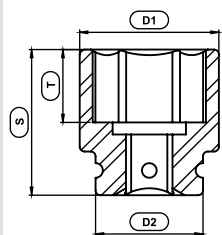
6pt. STD Socket
