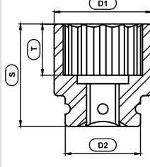
12t. STD Socket
