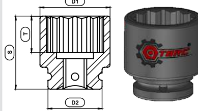
12t. STD Socket
