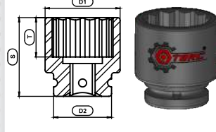
12pt. STD Socket
