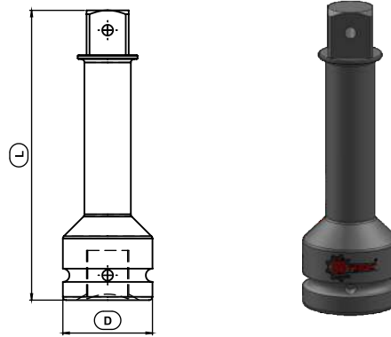
Extension Bar
