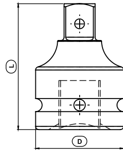
Adapter (Female - Male)
