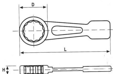
STRAIGHT RING TYPE SLUGGING WRENCH
